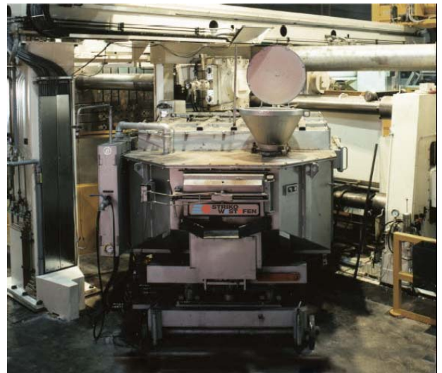
The ProDos® pouring an engine block, so efficient you can hold your hand on the furnace
